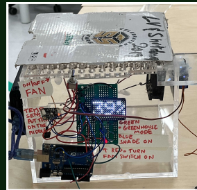
Automated Greenhouse (Hackathon 2024)
